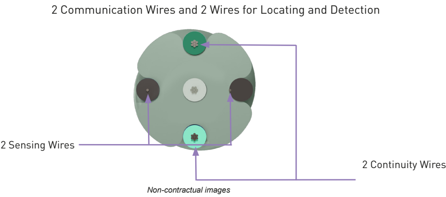
FG-ACSB Sense Cable Cutting View (without External Braid)
