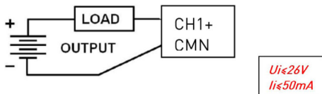
Figure 2: Single-output wiring
